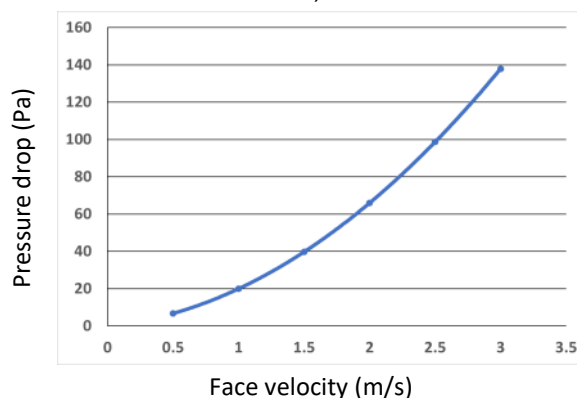
Performance: airflow, louver with insect mesh
