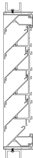
Typical detail
