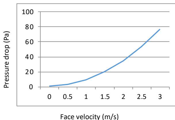
Performance: airflow, louvre with insect mesh
